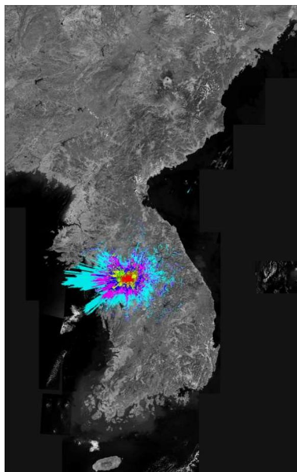
DMB Antenna Simulation
